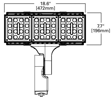
Direct Pole Mount
